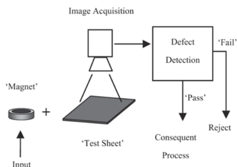
Figure 1. Automated Visual Inspection System
