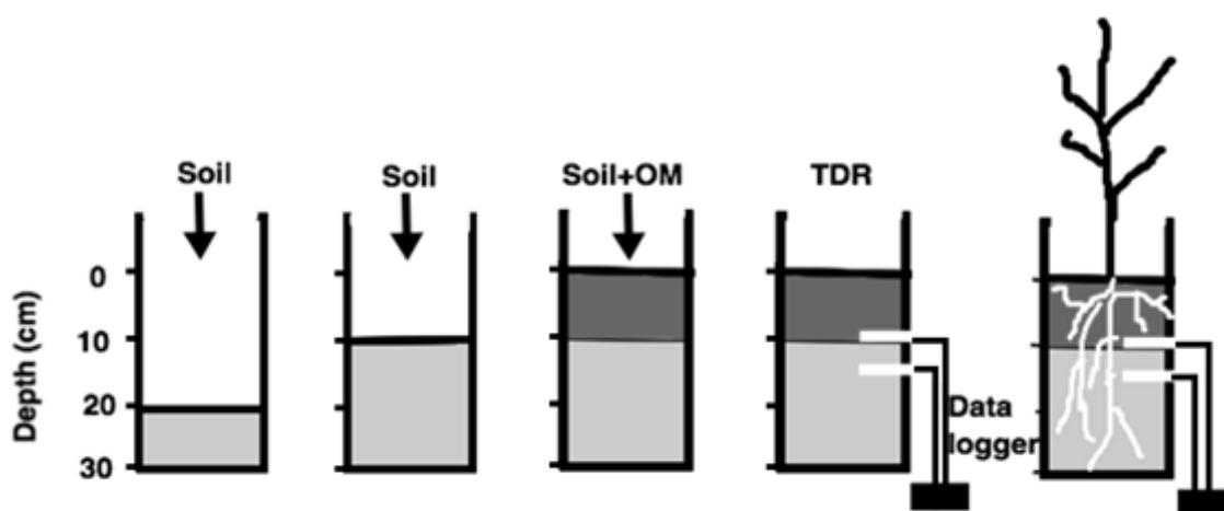
Figure 1 Mains steps of column filling, note that OM is incorporated only in the upper layer (0-10 cm depth). TDR probes were inserted at 10 and 15 cm in one column. The last drawing is a schematically presentation of maize shoots and roots.
