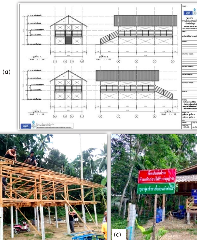
Figure 6 Goat housing; (a) Plan for the goat house, (b) Building the goat shelter, and (c) Group goat house
