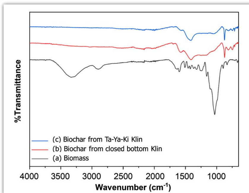
Figure 5 FTIR spectra of; (a) Biomass, (b) Biochar from closed bottom kiln, and (c) Biochar from Ta-Ya-Ki kiln
