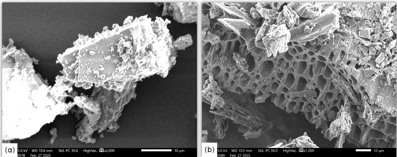
Figure 6 SEM morphology of; (a) Biochar from closed bottom kiln and (b) Biochar from Ta-Ya-Ki kiln
